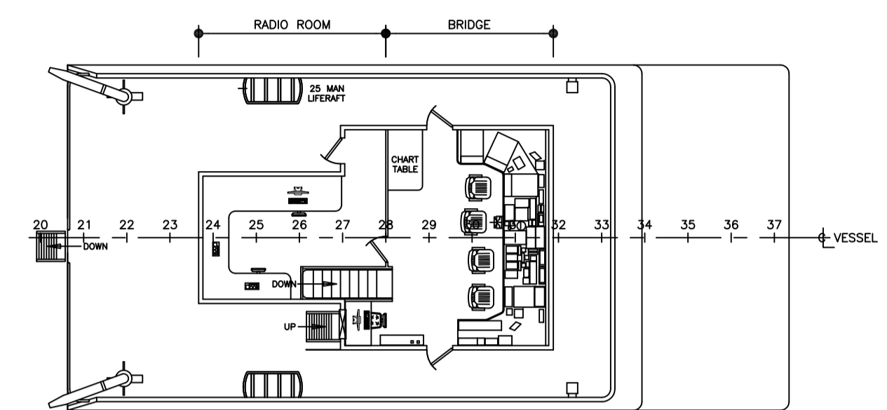
WHEELHOUSE DECK
