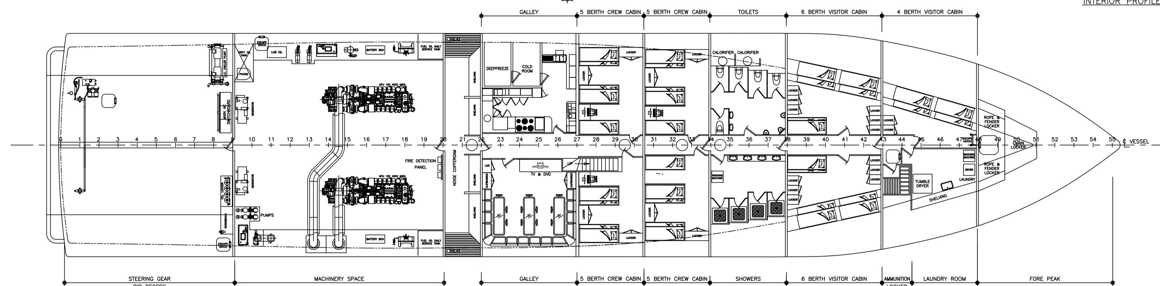
LOWER DECK
