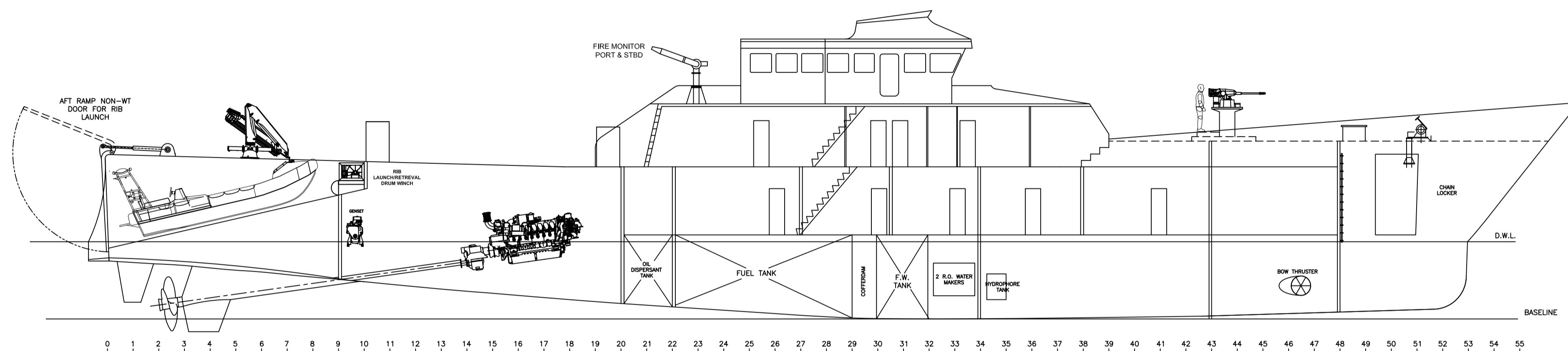
INTERIOR PROFILE
