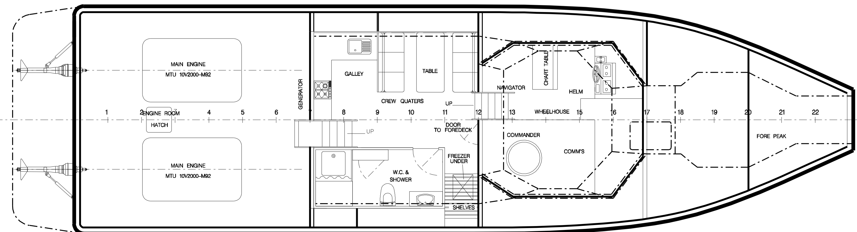
DECK PLAN
