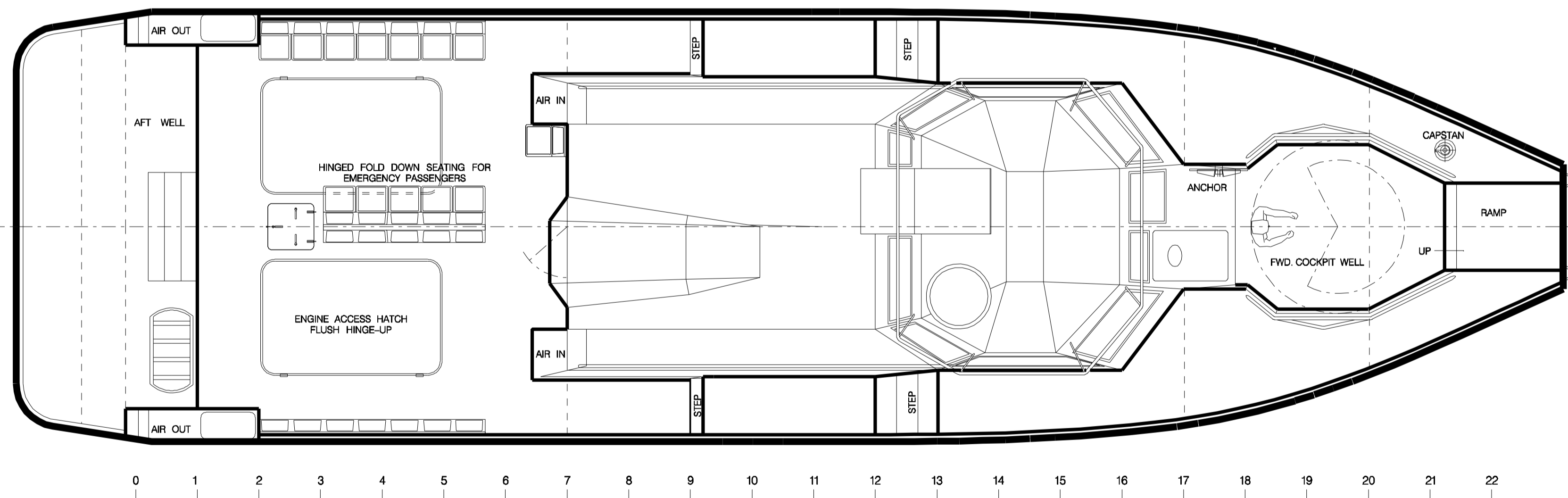
INBOARD PROFILE
