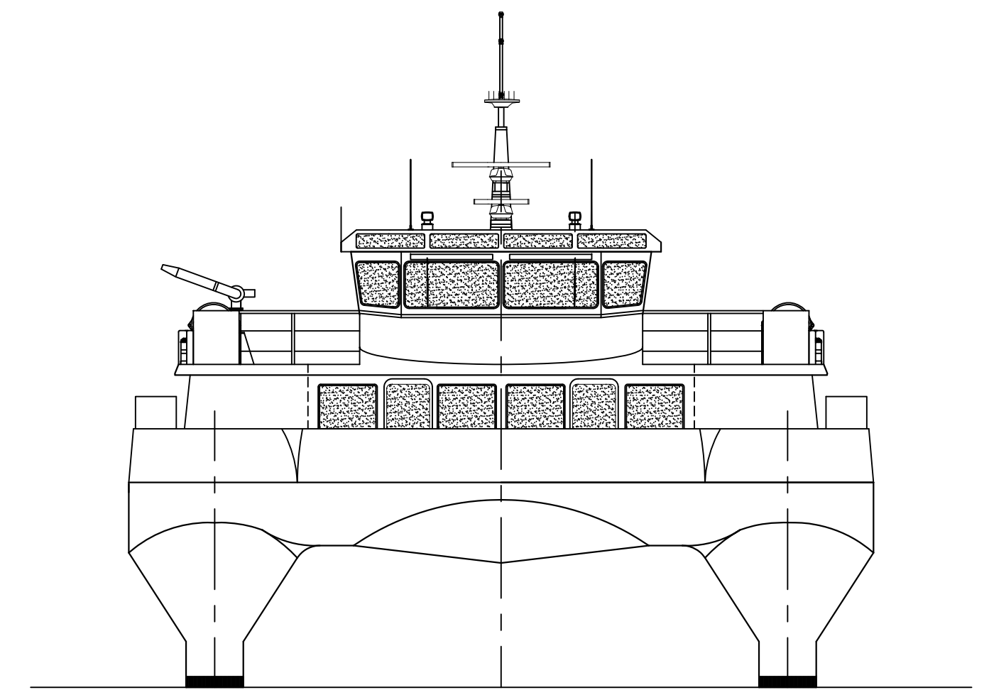
BOW VIEW (LOOKING AFT)
